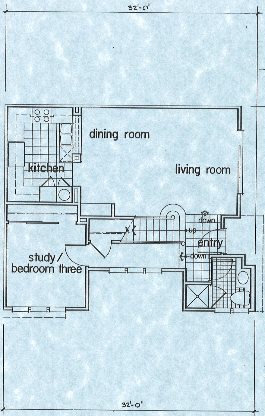
① plan C first floor
