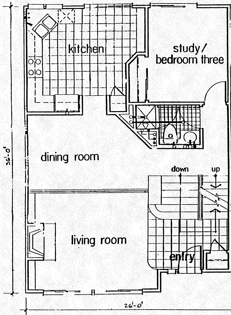
plan B first floor
