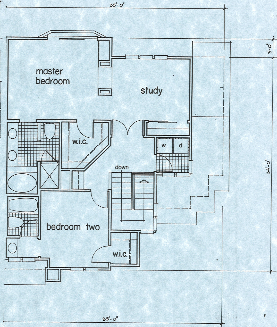
② plan A second floor
