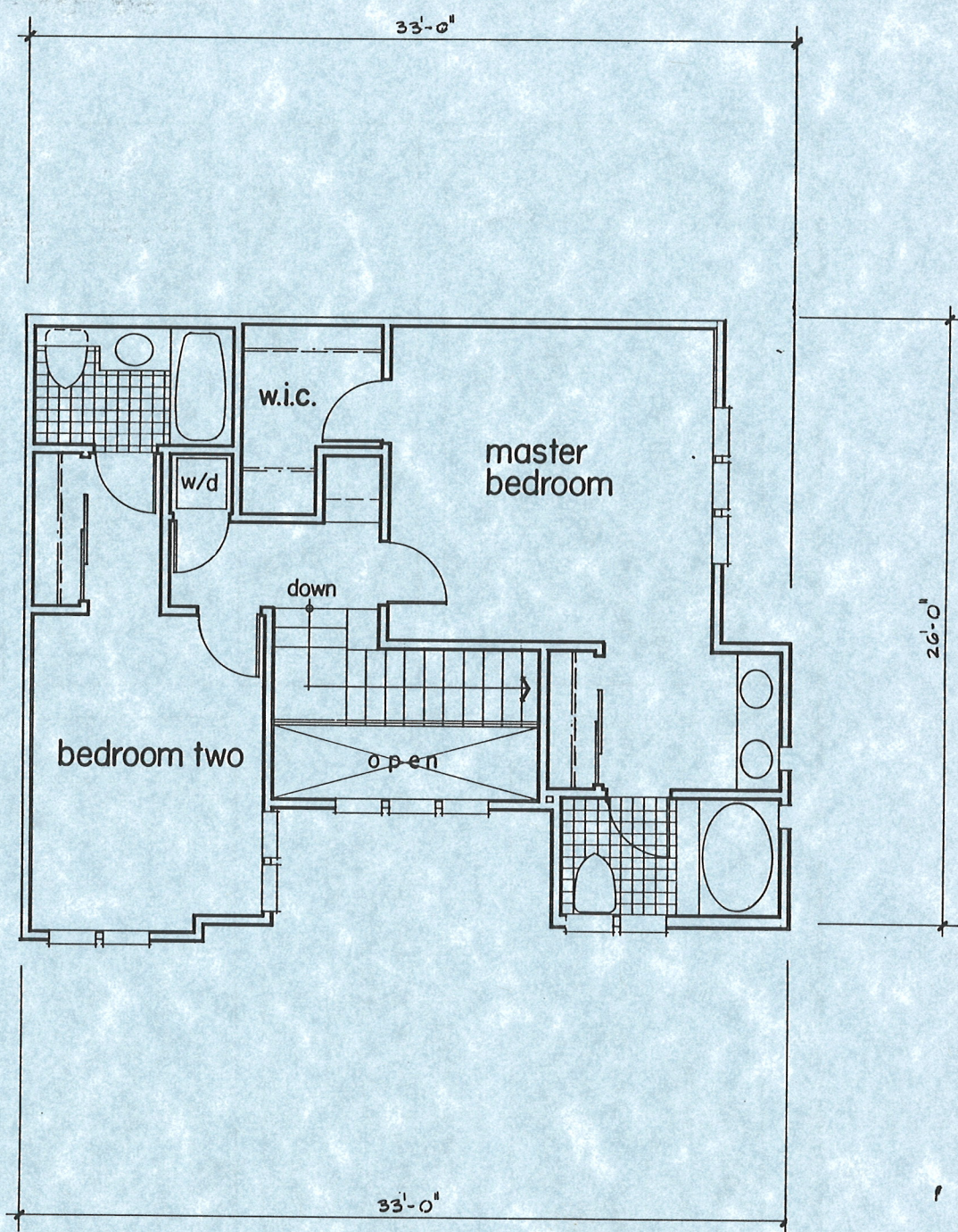
② plan C second floor
