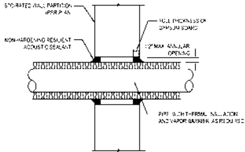
Pipe Penetrations at STC-Rated Partitions (STC45 and higher)
